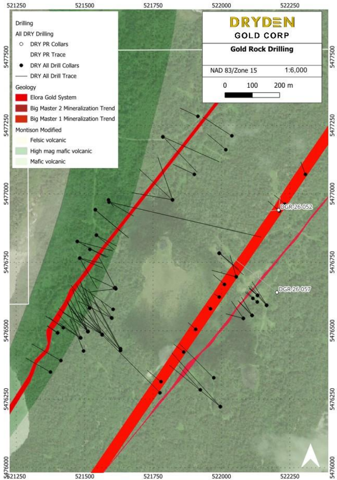
Drill hole location map with highlighted labels June 2 nd 2026 release
