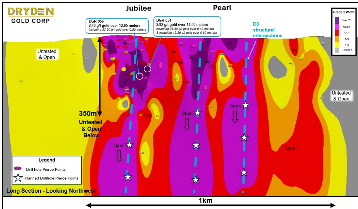
Figure 4: Long Section Elora Gold System – Jubilee and Pearl Target Mining Hub Link- https://mininghub.com/3d/v/6dcjgqzm
