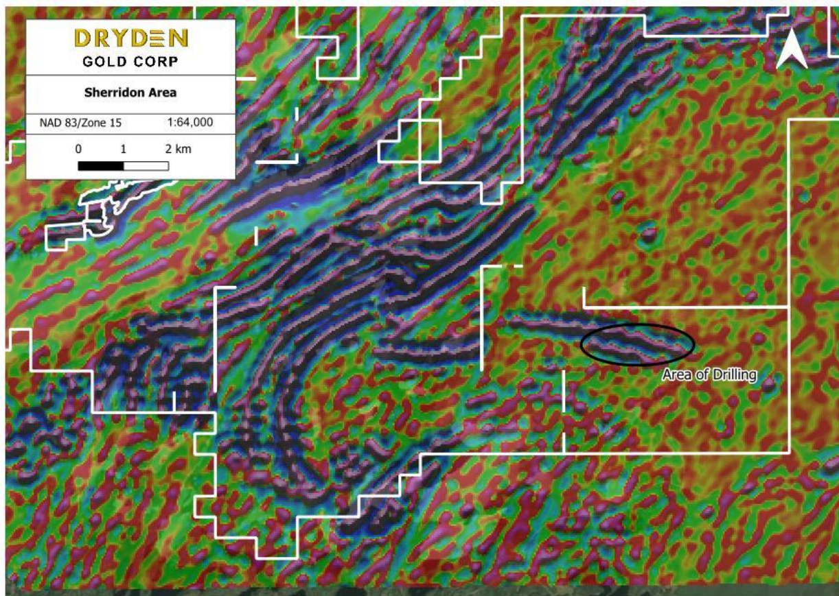
Plan map of the Sherridon with 2 nd Derivative geophysics demonstrating the strike length potential of the deep-rooted ultramafic intrusions (magnetic highs trending E-W).
