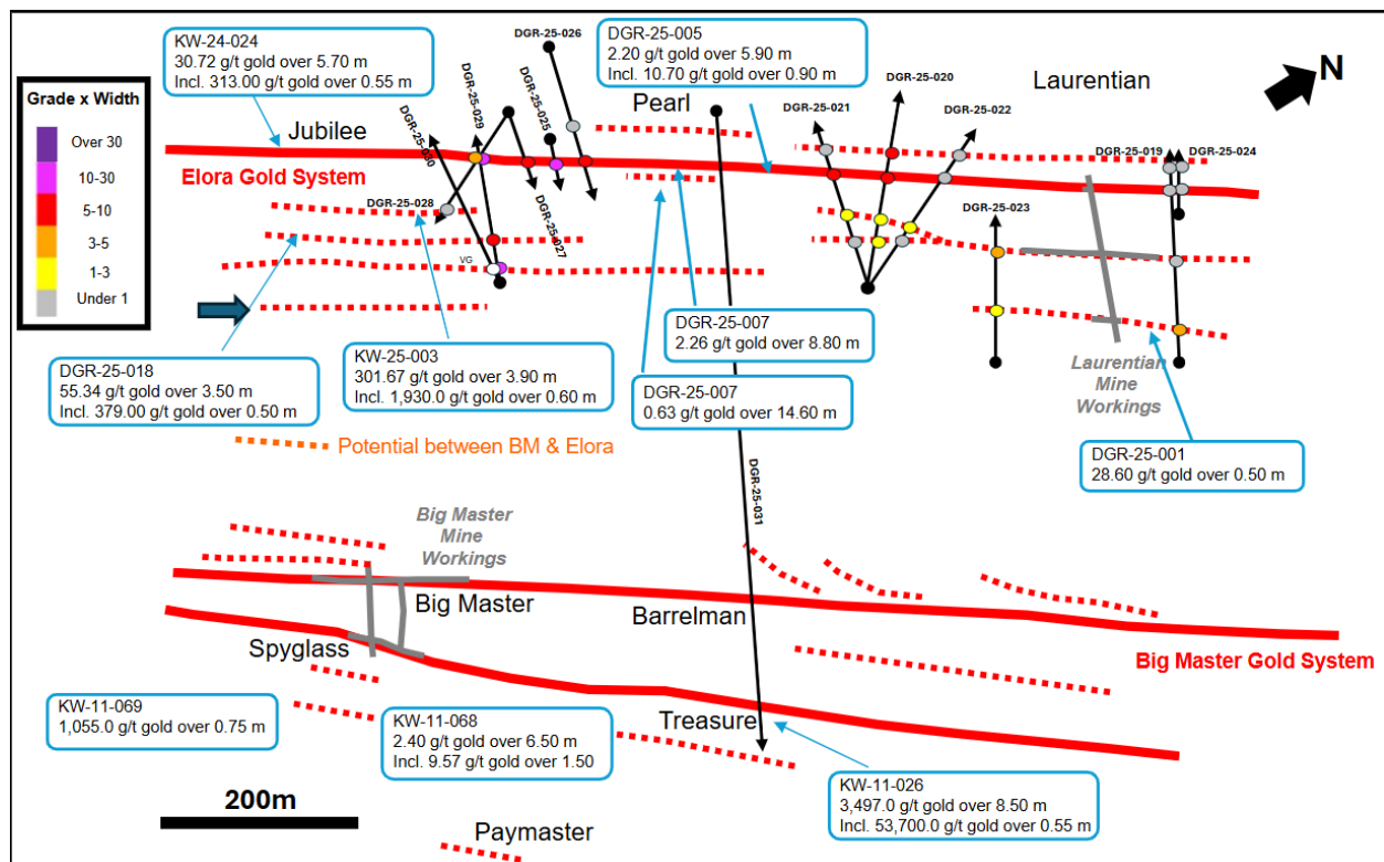
Illustrated oblique Plan View of Gold Rock showing mineralized structures and various hole locations.
